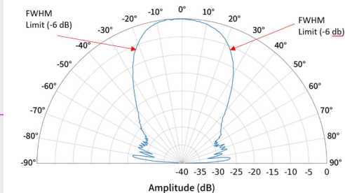
Figure 6. A beam pattern of a 45-degree FoV horn measured against a large flat target.
